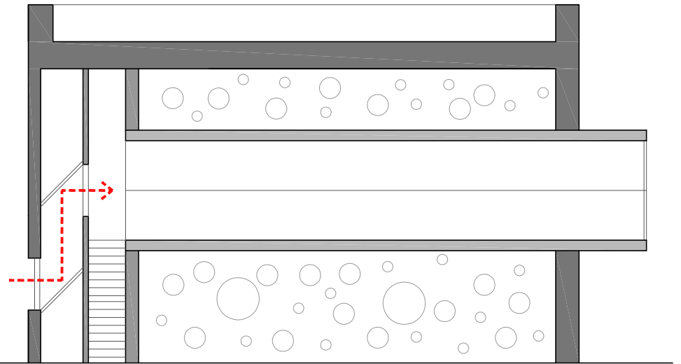
Section
