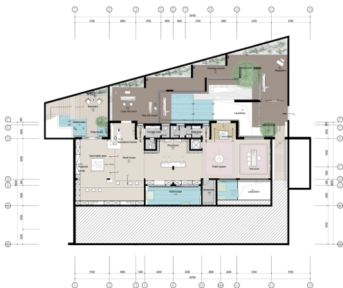
Floor plan of the negative one floor
