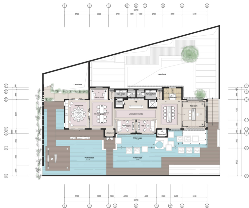
Floor plan of the first floor
